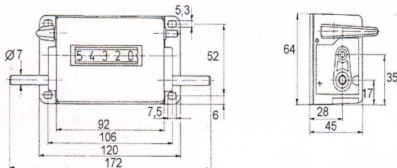
Dimensions M400/M410
